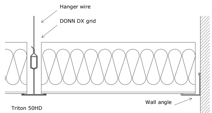
Detail: Triton 50HD ceiling tiles suspended on Rondo Donn® DX Grid
