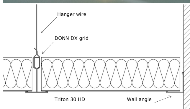
Detail: Triton 30HD ceiling tiles suspended on Rondo Donn DX Grid
