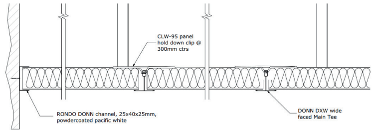
Technical Drawing
